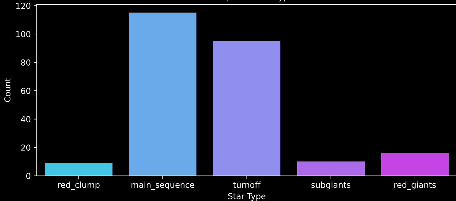
GALAH DR4 Field: [1645] Count plot of Star Type
