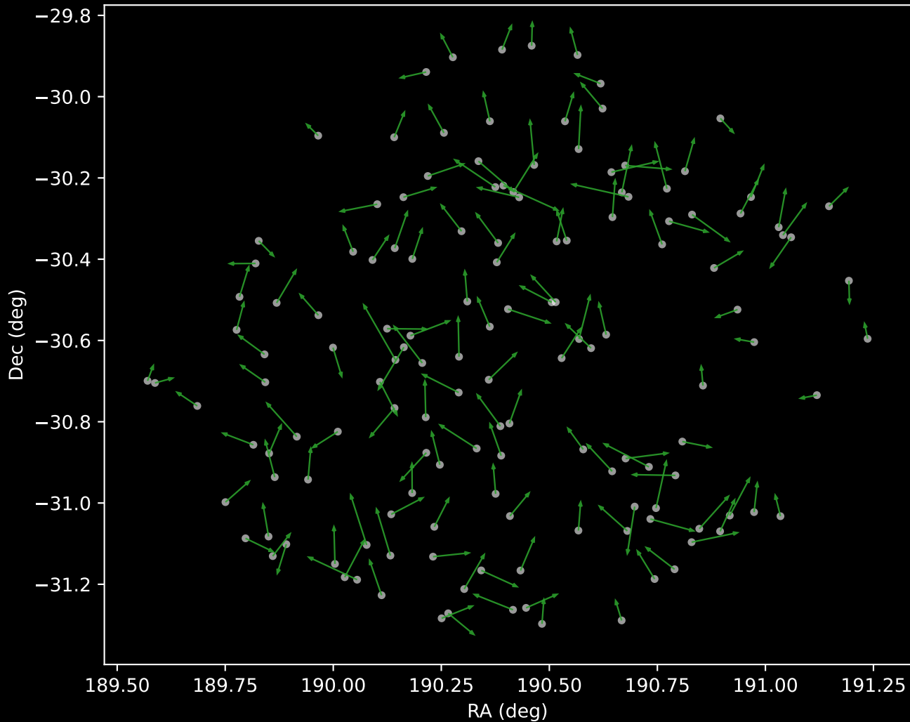
GALAH DR4 Cluster 4 Proper Motion Vectors (n=144)
