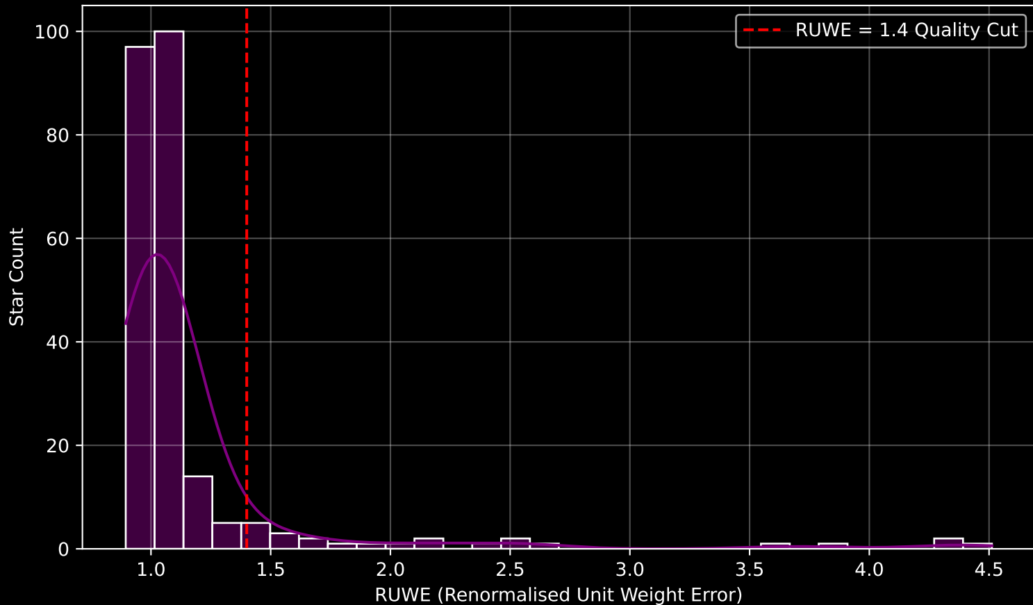
GALAH DR4 Field [1645] RUWE Distribution (n= 240)
